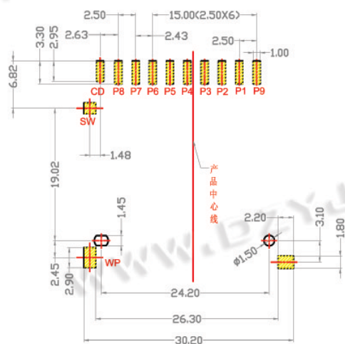
P. C. B LAYOUT
